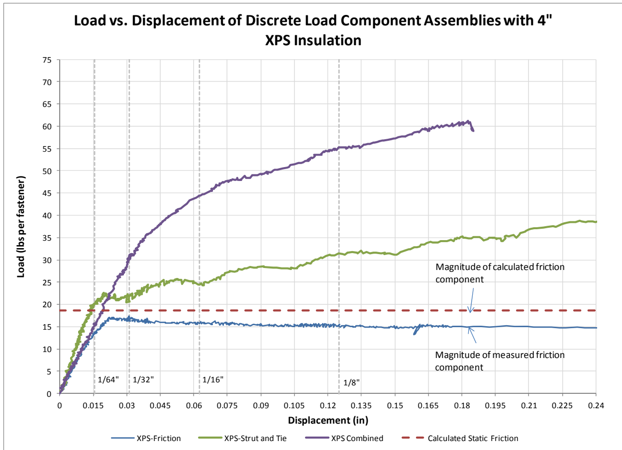
Figure 30. Measured versus calculated friction load component resistance
