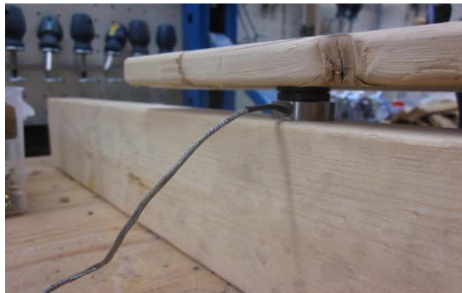
Figure 15. Precompression force test setup
