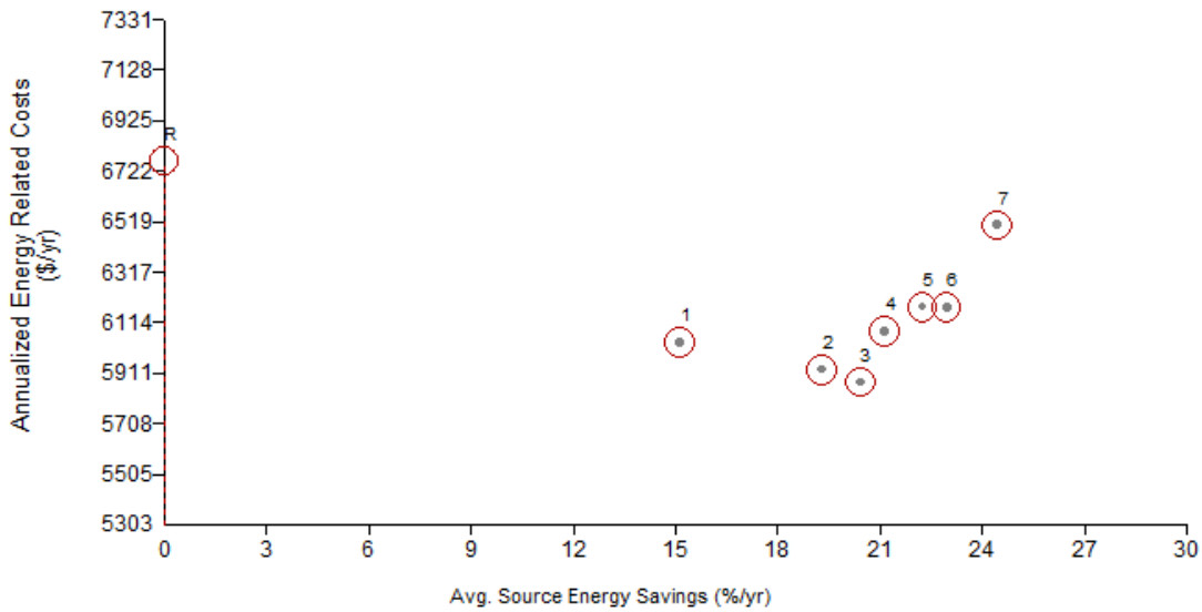
Figure 41. Annualized energy-related costs versus average source energy savings for Boston
