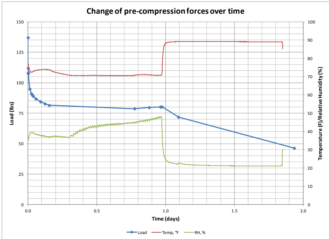
Figure 31. Change of precompression forces over time
