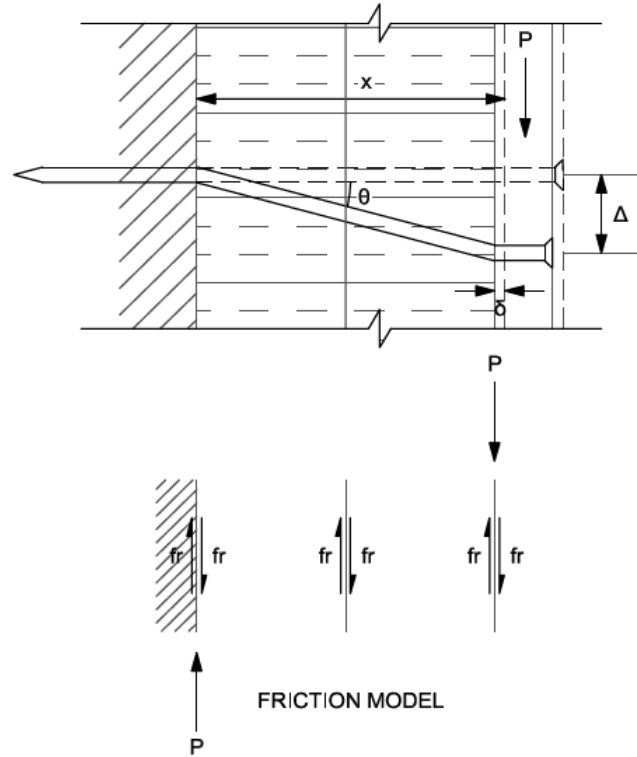
Figure 11. Free body diagram of the friction resistance between material layers
