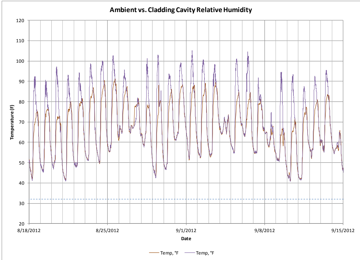
Figure 32. Sample of ambient versus cladding cavity temperatures
