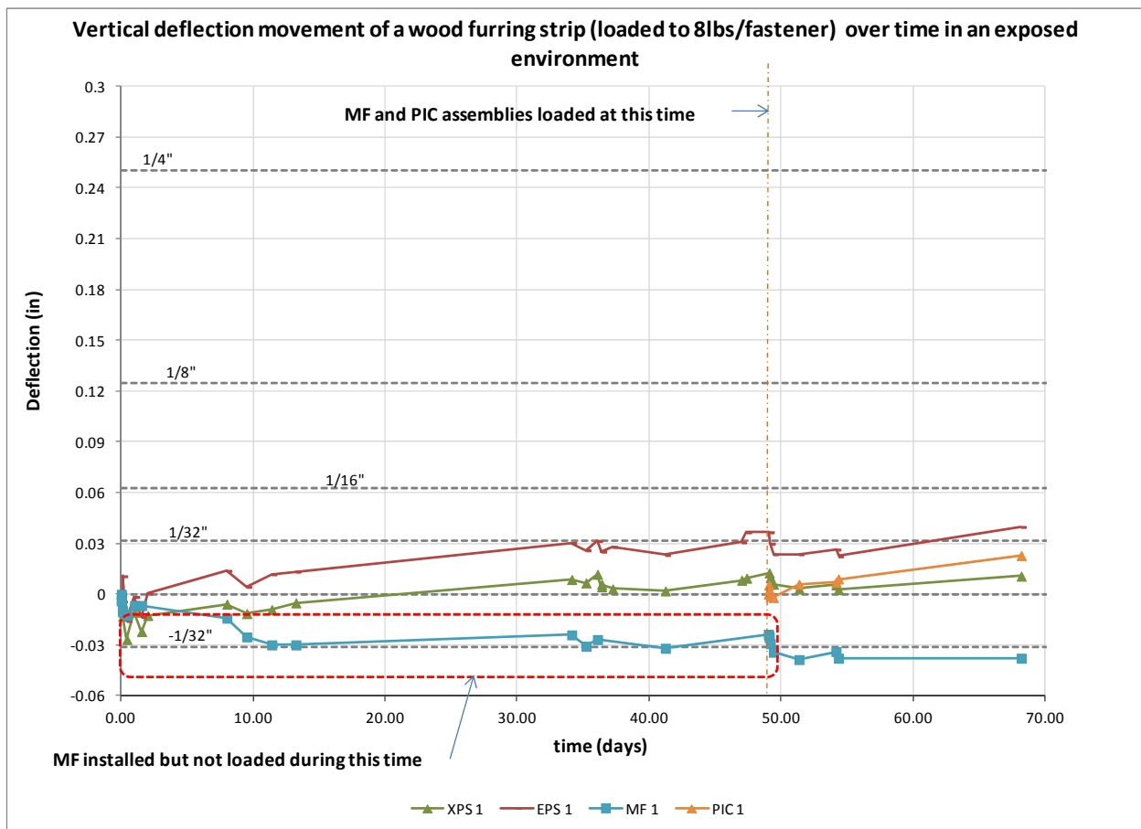
Figure 24. Long-term environmental exposure of lightweight claddings
