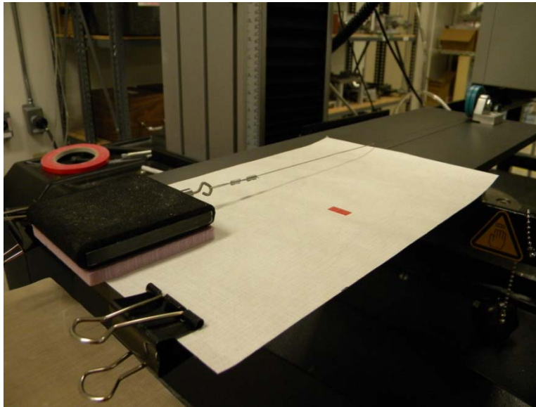
Figure 14. Example of a static COF test
