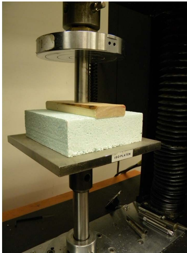
Figure 13. Example of insulation compression Test B
