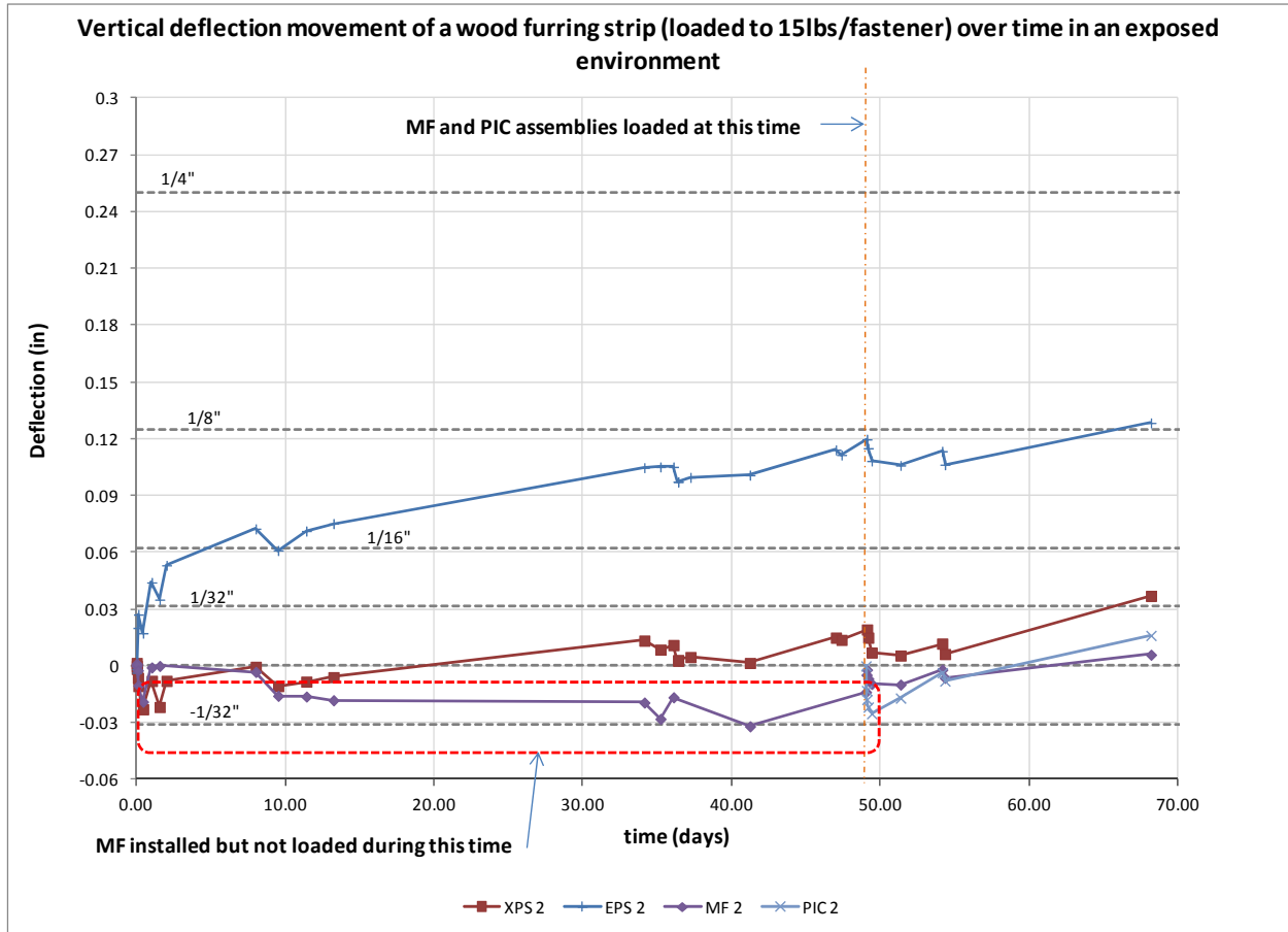
Figure 25. Long-term environmental exposure of medium-weight claddings
