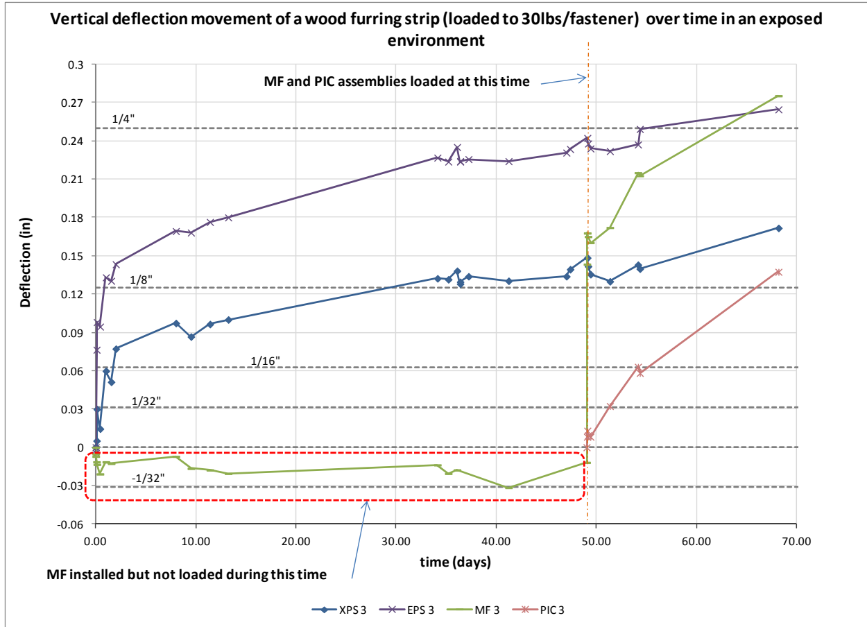
Figure 26. Long-term environmental exposure of heavyweight claddings
